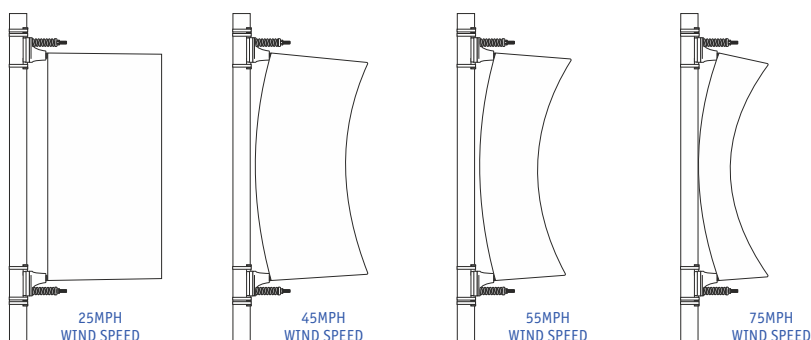
DIAGRAM TO SHOW THE WIND SPILL OF THE BANNERSPRING.
