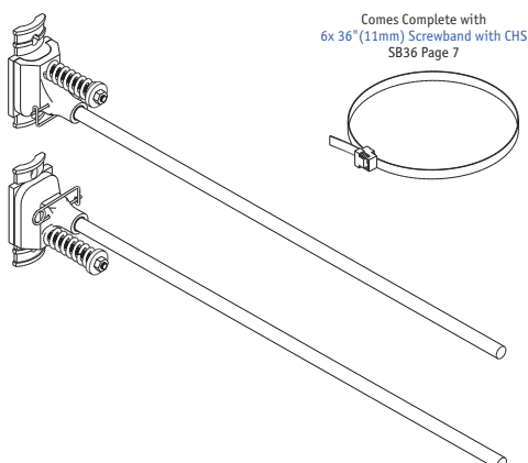
BannerSpring Bracket (Suitable for banners up to 700mm x 3000mm) SPRINGB
